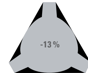
Comparison of cross-section: Standard triangle (outside) and EcoStar® (inside)
